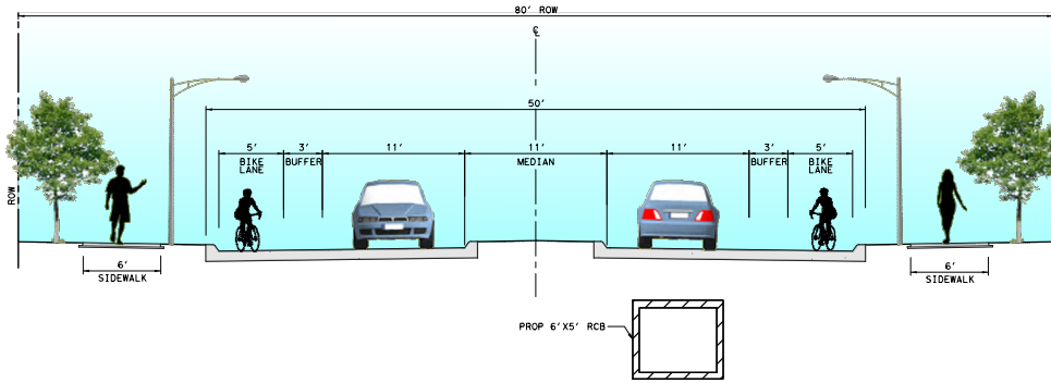
PROPOSED SECTION AT W43RD NEAR SUE BARNETT
