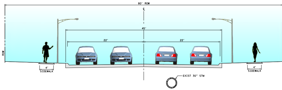
EXISTING SECTION AT W43RD NEAR SUE BARNETT
