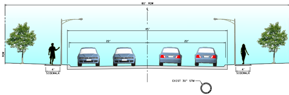
EXISTING SECTION AT W43RD BETWEEN SUE BARNETT AND SHEPHERD
