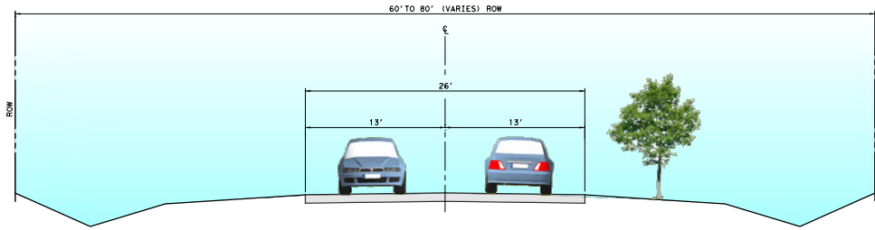
EXISTING SECTION AT SUE BARNETT SOUTH OF WEST 41ST
